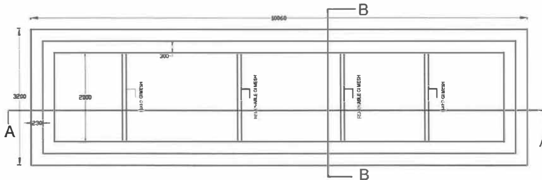
PLAN OF HORIZONTAL ROUGHING FILTER
