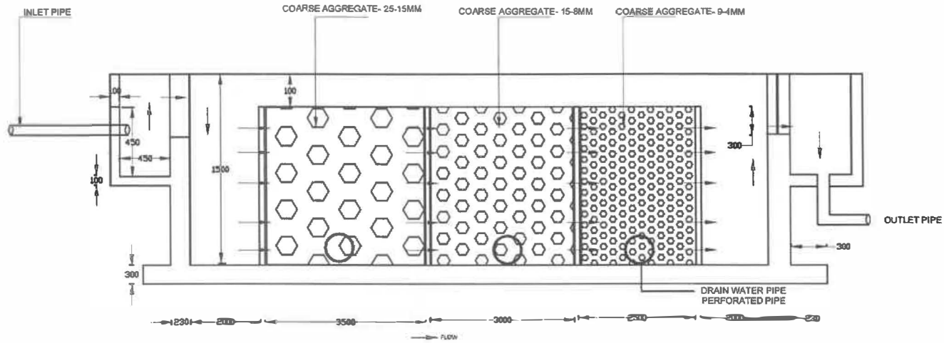
SECTION OF HORIZONTAL ROUGHING FILTER
